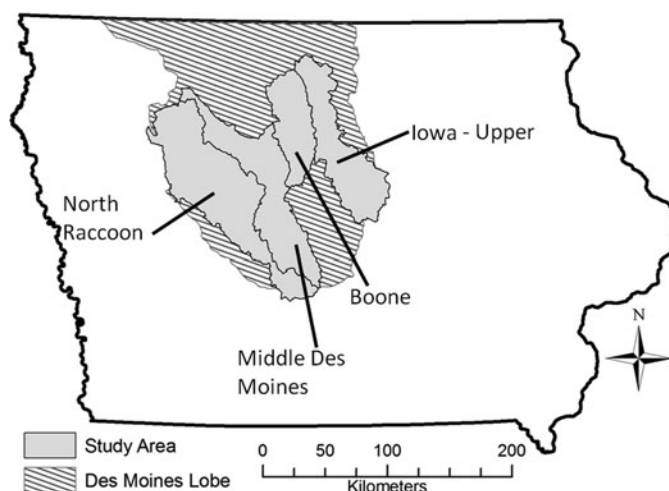
FIGURE 1. Location of eight-digit hydrological unit code (HUC8) study basins within the Des Moines Lobe subcoregion of Iowa.
